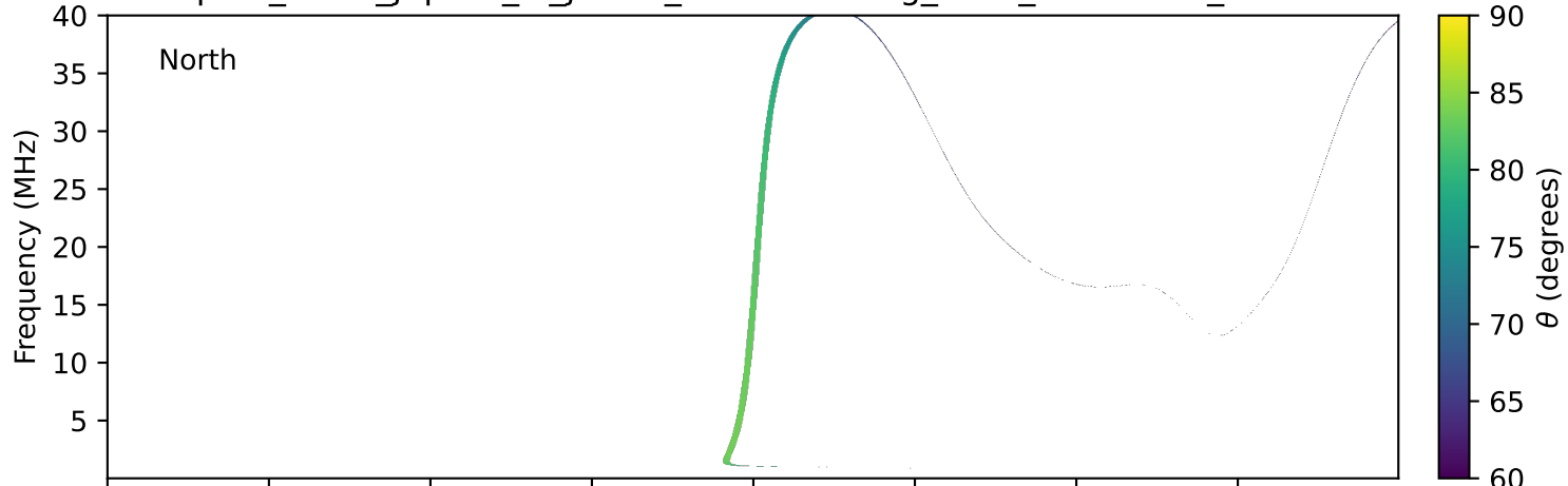
expres_earth_jupiter_io_jrm33_lossc-wid1deg_3kev_20211006_v11.cdf
