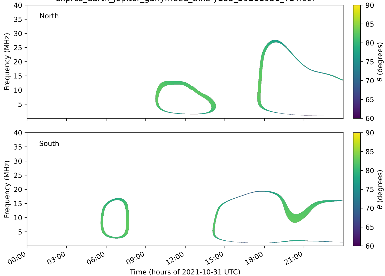
expres_earth_jupiter_ganymede_txka-y235_20211031_v14.cdf
