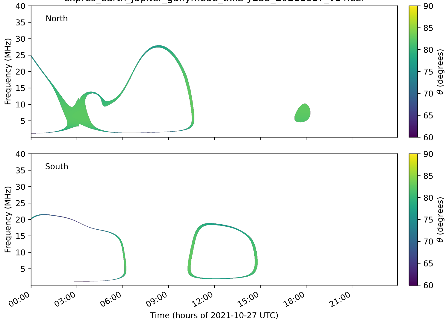
expres_earth_jupiter_ganymede_txka-y235_20211027_v14.cdf
