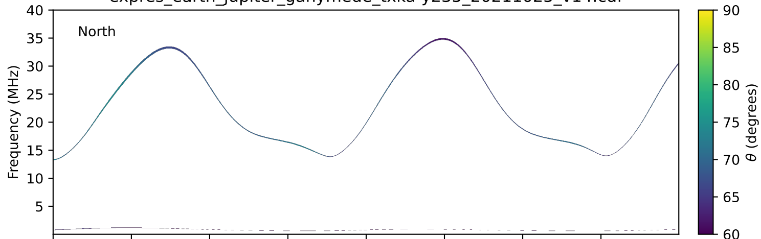
expres_earth_jupiter_ganymede_txka-y235_20211025_v14.cdf
