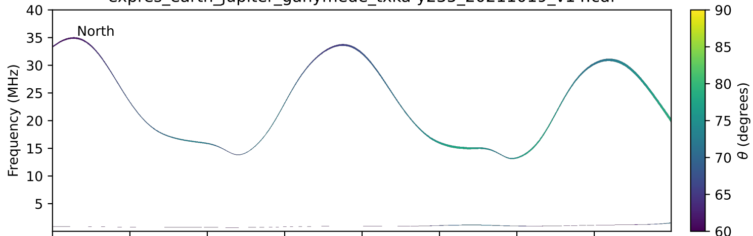
expres_earth_jupiter_ganymede_txka-y235_20211019_v14.cdf
