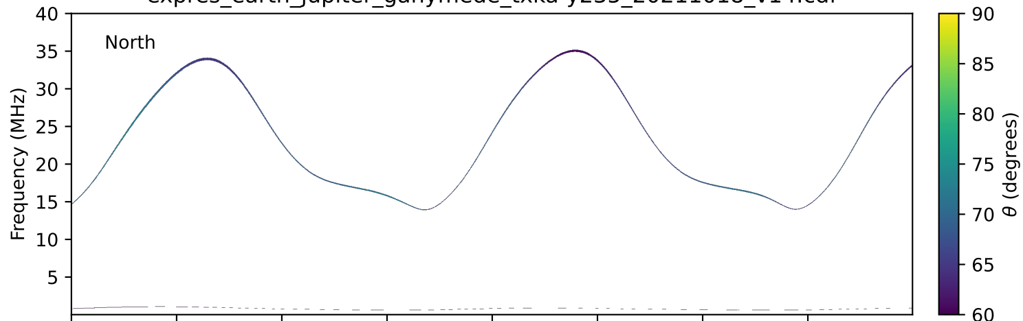
expres_earth_jupiter_ganymede_txka-y235_20211018_v14.cdf
