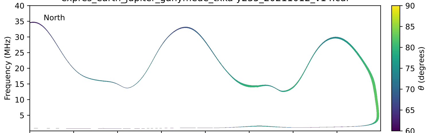
expres_earth_jupiter_ganymede_txka-y235_20211012_v14.cdf
