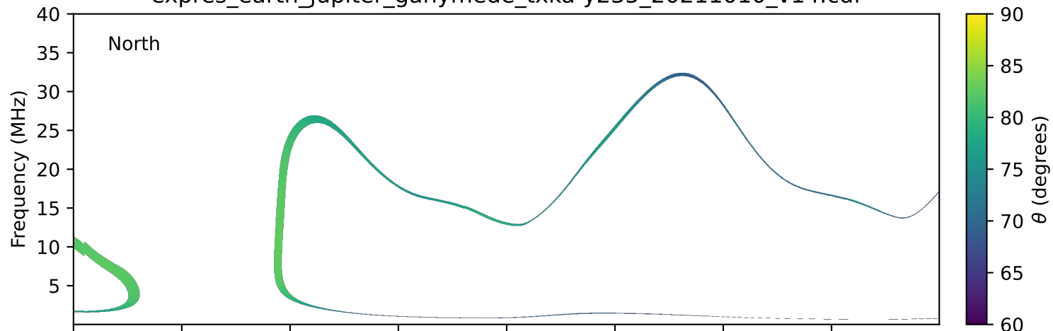
expres_earth_jupiter_ganymede_txka-y235_20211010_v14.cdf
