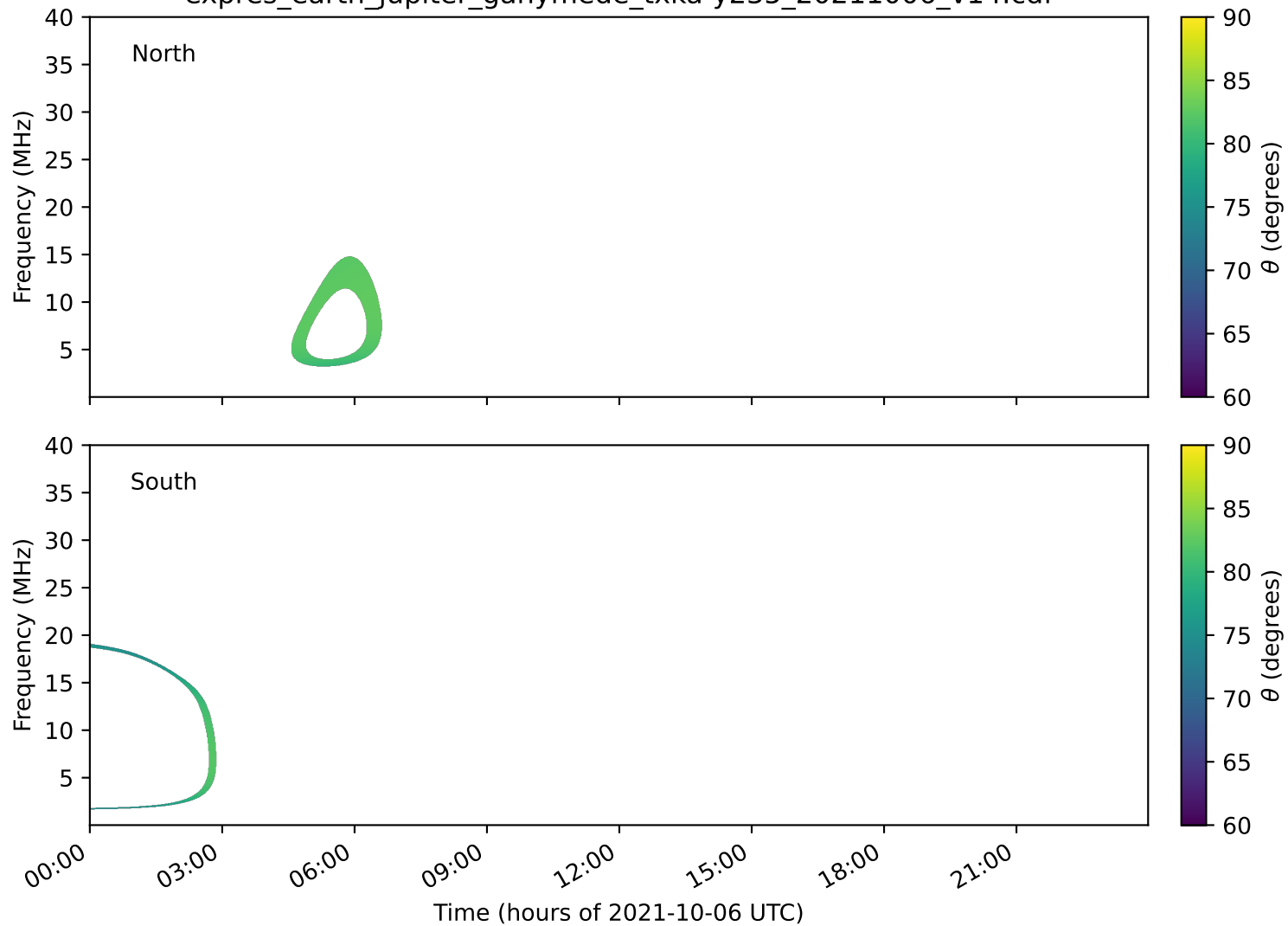
expres_earth_jupiter_ganymede_txka-y235_20211006_v14.cdf
