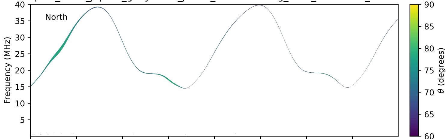
expres_earth_jupiter_ganymede_jrm33_lossc-wid1deg_3kev_20211025_v11.cdf
