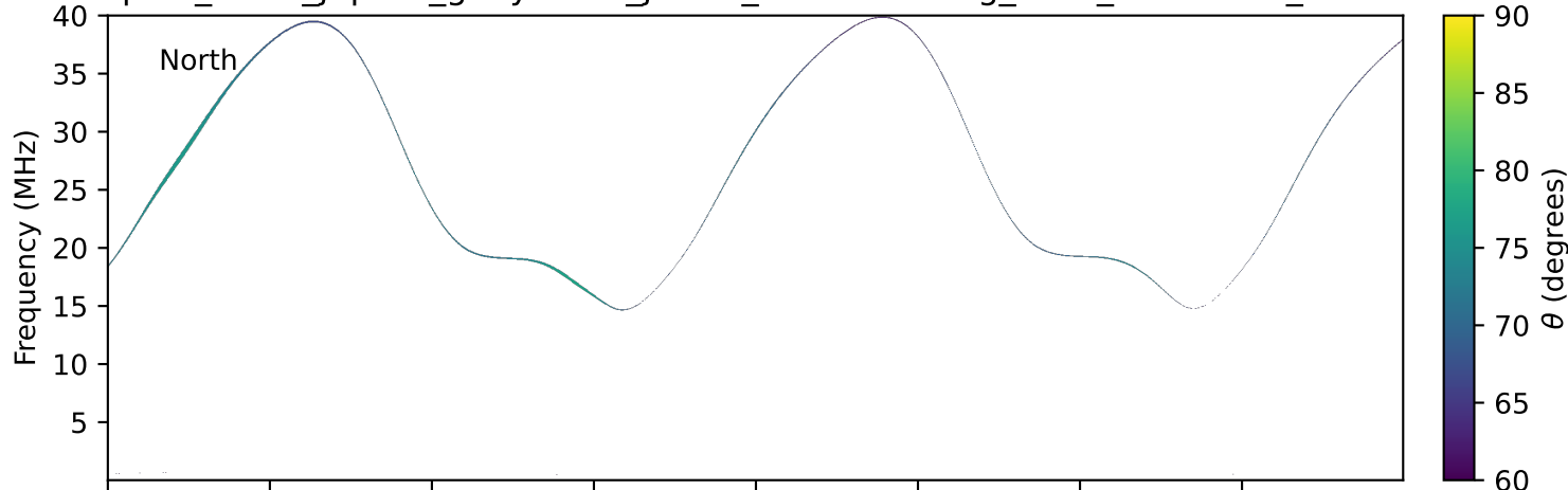
expres_earth_jupiter_ganymede_jrm33_lossc-wid1deg_3kev_20211018_v11.cdf
