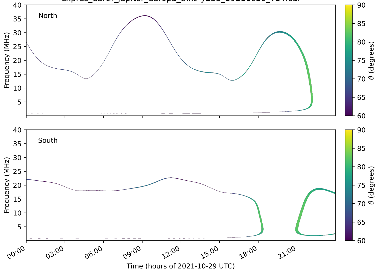
expres_earth_jupiter_europa_txka-y235_20211029_v14.cdf
