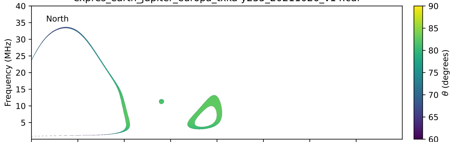
expres_earth_jupiter_europa_txka-y235_20211026_v14.cdf
