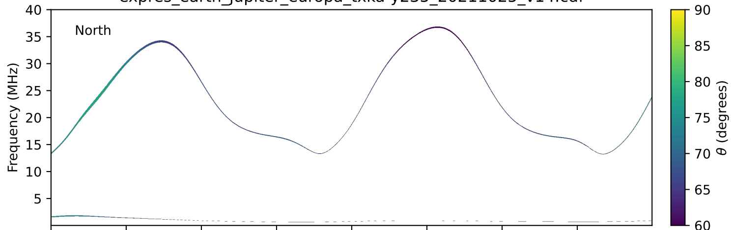
expres_earth_jupiter_europa_txka-y235_20211025_v14.cdf
