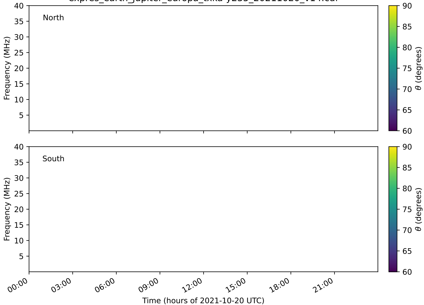
expres_earth_jupiter_europa_txka-y235_20211020_v14.cdf
