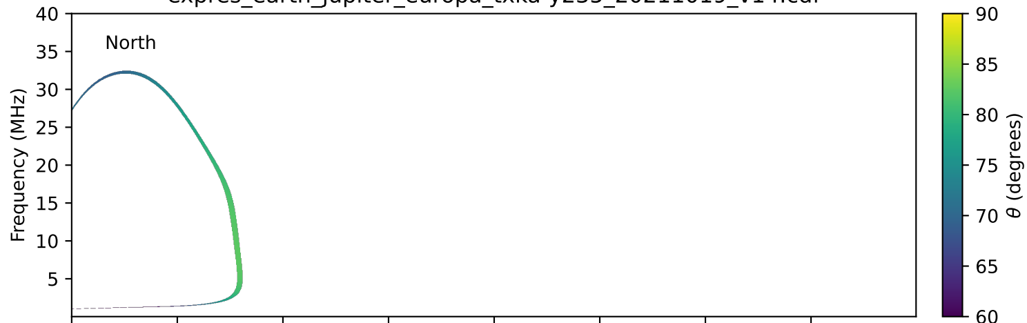
expres_earth_jupiter_europa_txka-y235_20211019_v14.cdf
