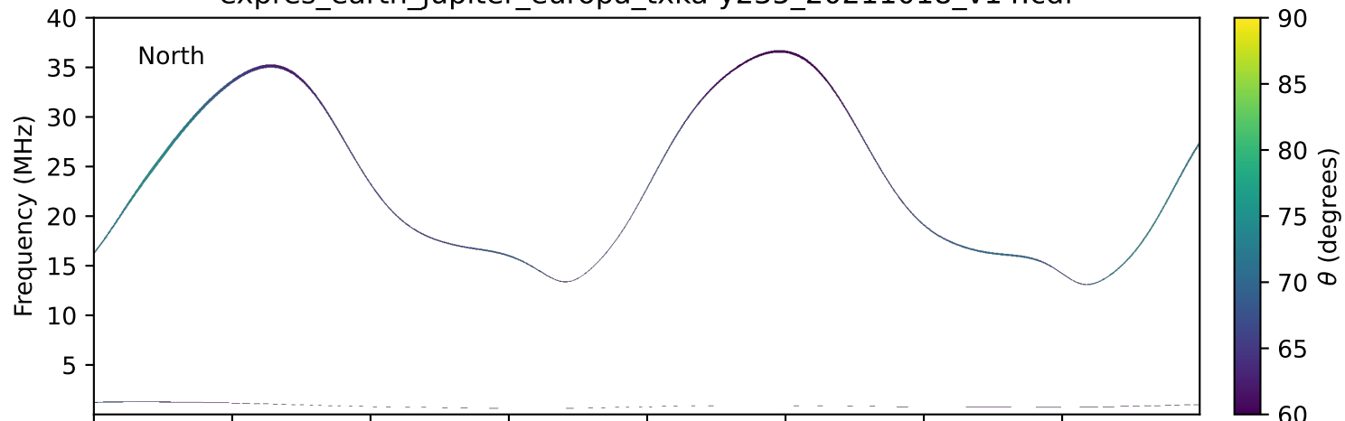
expres_earth_jupiter_europa_txka-y235_20211018_v14.cdf
