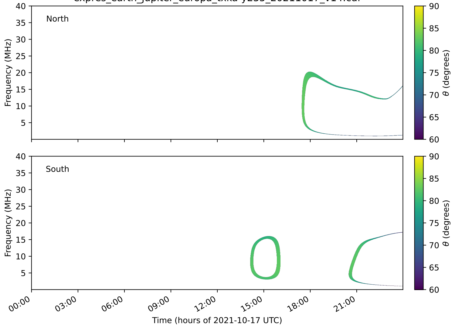
expres_earth_jupiter_europa_txka-y235_20211017_v14.cdf
