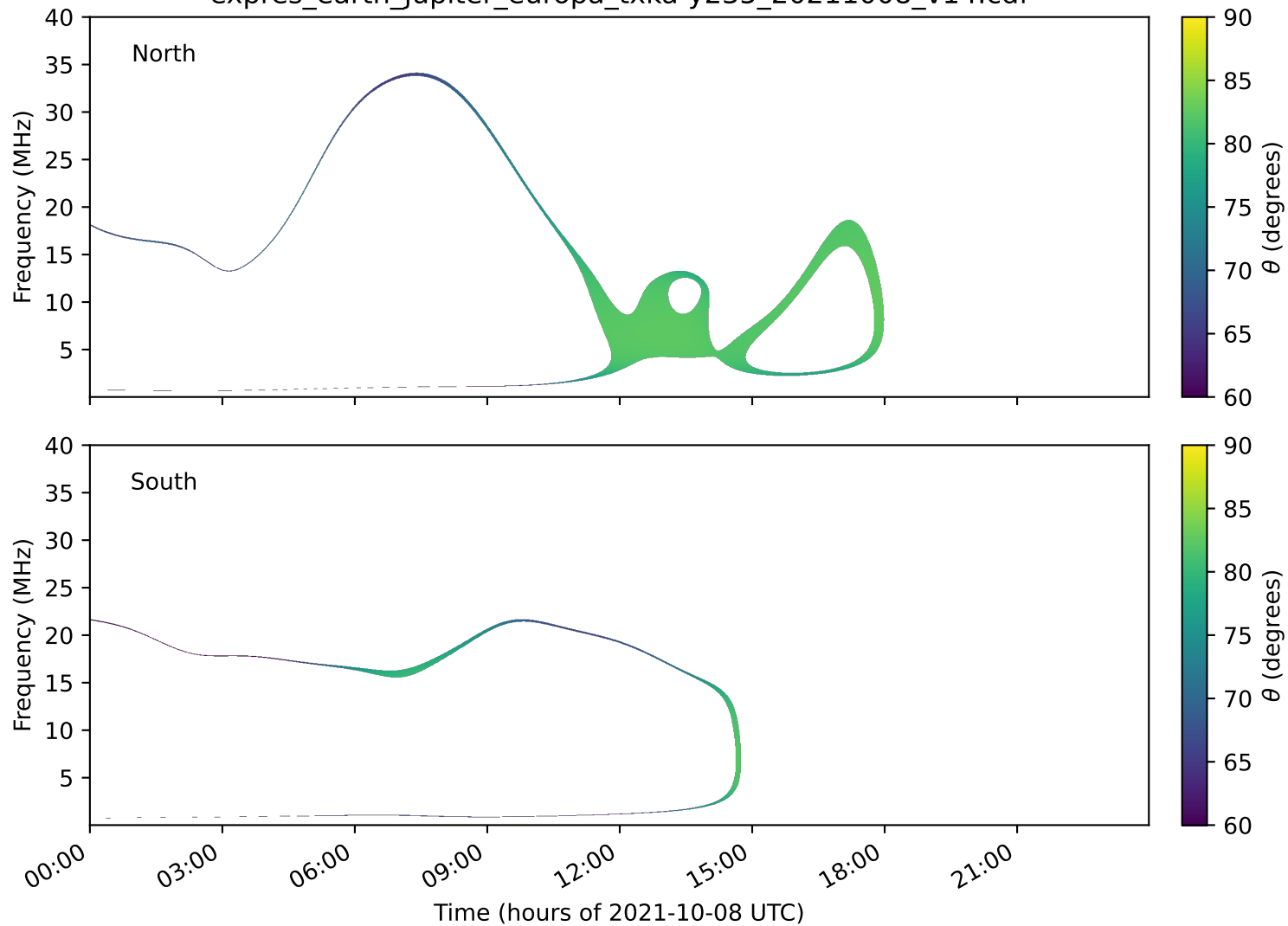
expres_earth_jupiter_europa_txka-y235_20211008_v14.cdf
