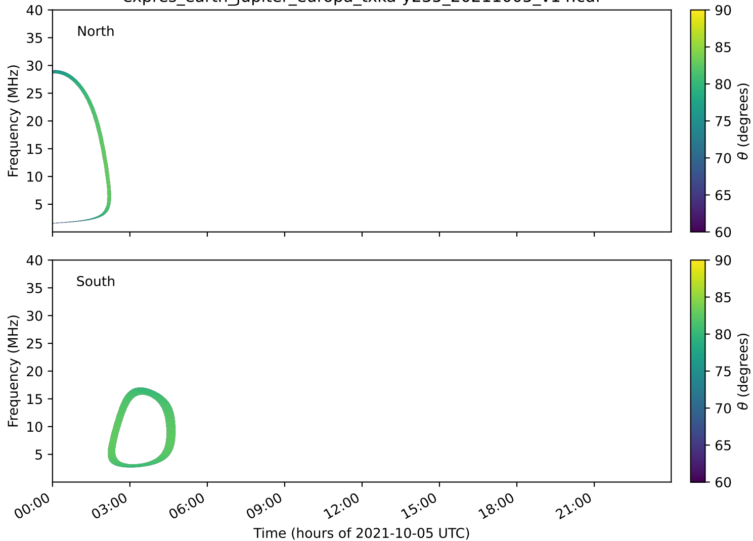
expres_earth_jupiter_europa_txka-y235_20211005_v14.cdf
