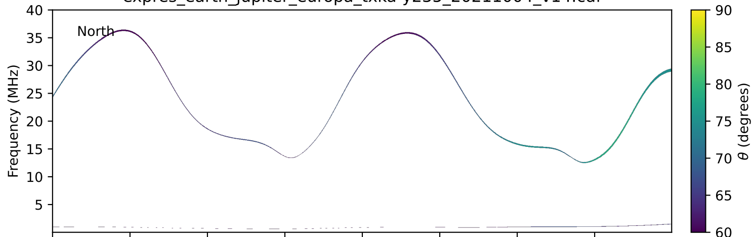
expres_earth_jupiter_europa_txka-y235_20211004_v14.cdf
