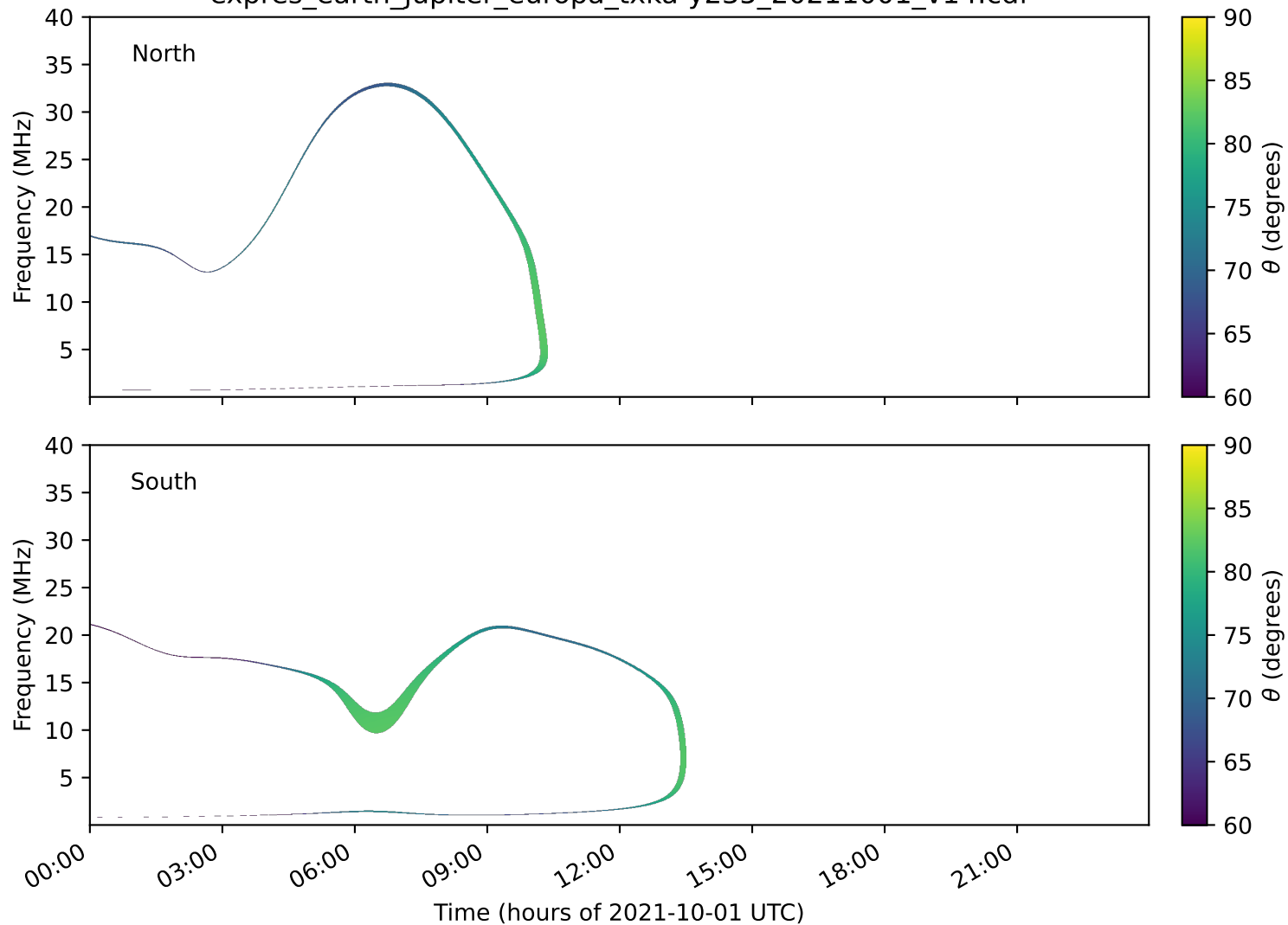
expres_earth_jupiter_europa_txka-y235_20211001_v14.cdf
