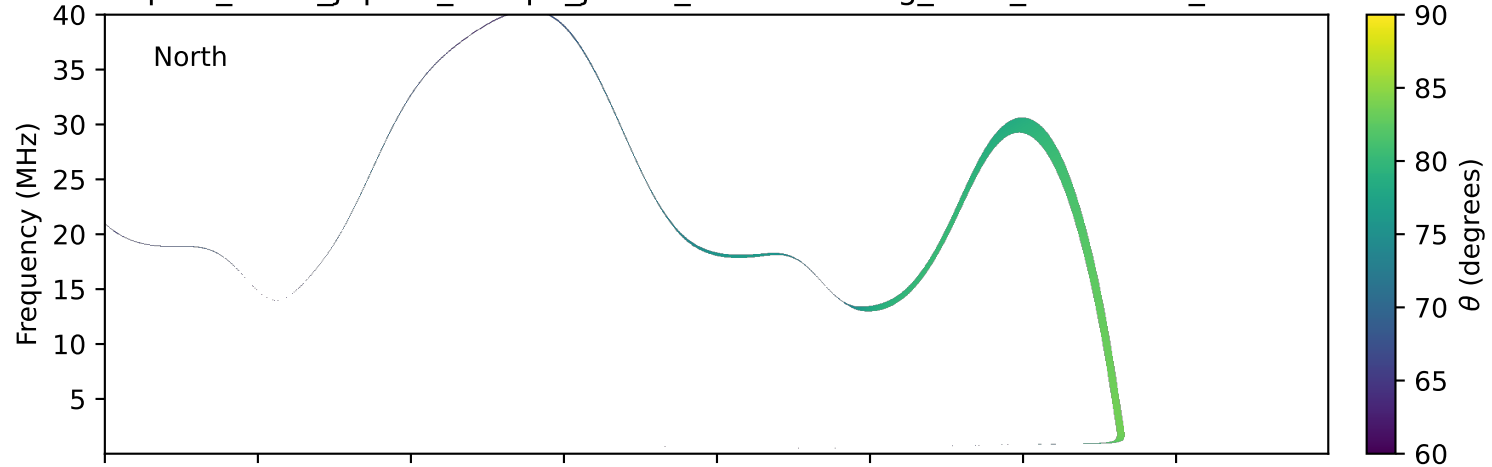
expres_earth_jupiter_europa_jrm33_lossc-wid1deg_3kev_20211015_v11.cdf
