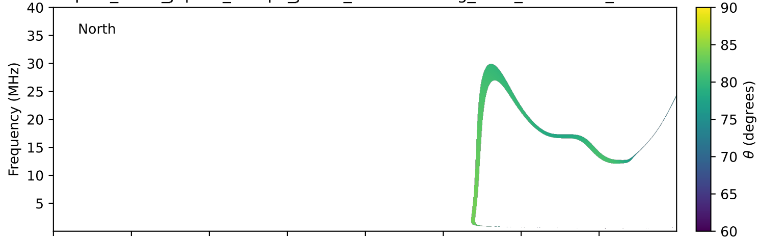
expres_earth_jupiter_europa_jrm33_lossc-wid1deg_3kev_20211010_v11.cdf
