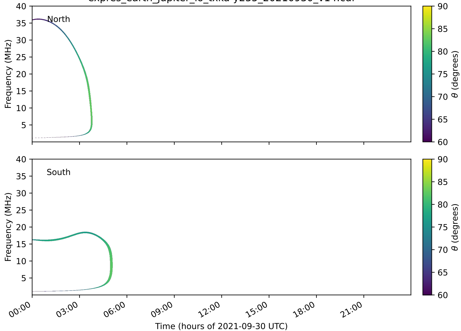
expres_earth_jupiter_io_txka-y235_20210930_v14.cdf
