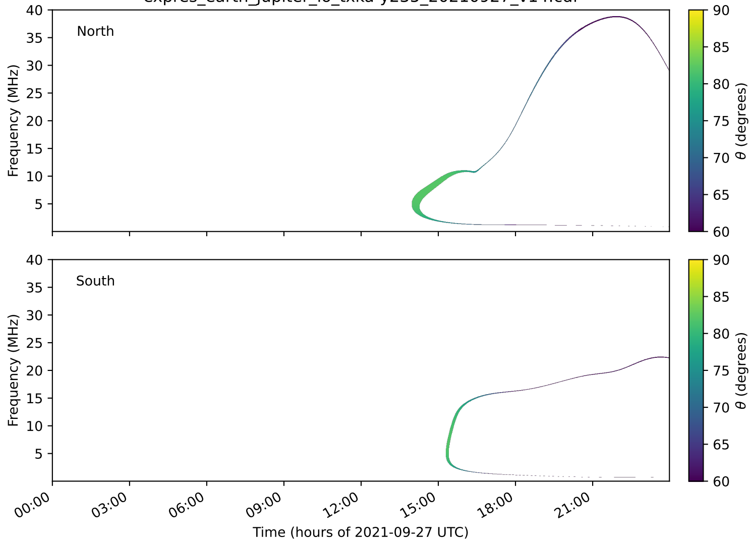
expres_earth_jupiter_io_txka-y235_20210927_v14.cdf
