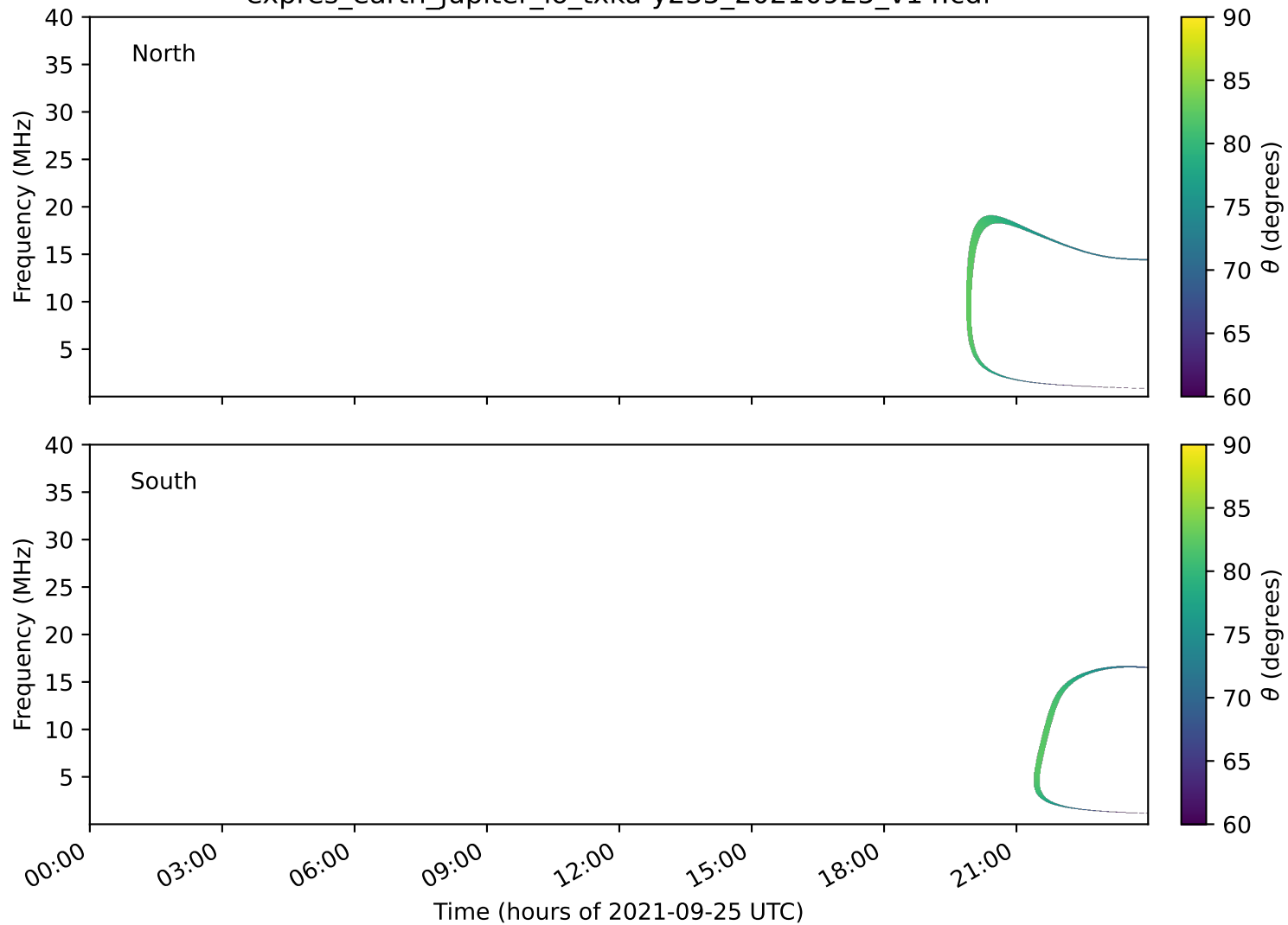
expres_earth_jupiter_io_txka-y235_20210925_v14.cdf
