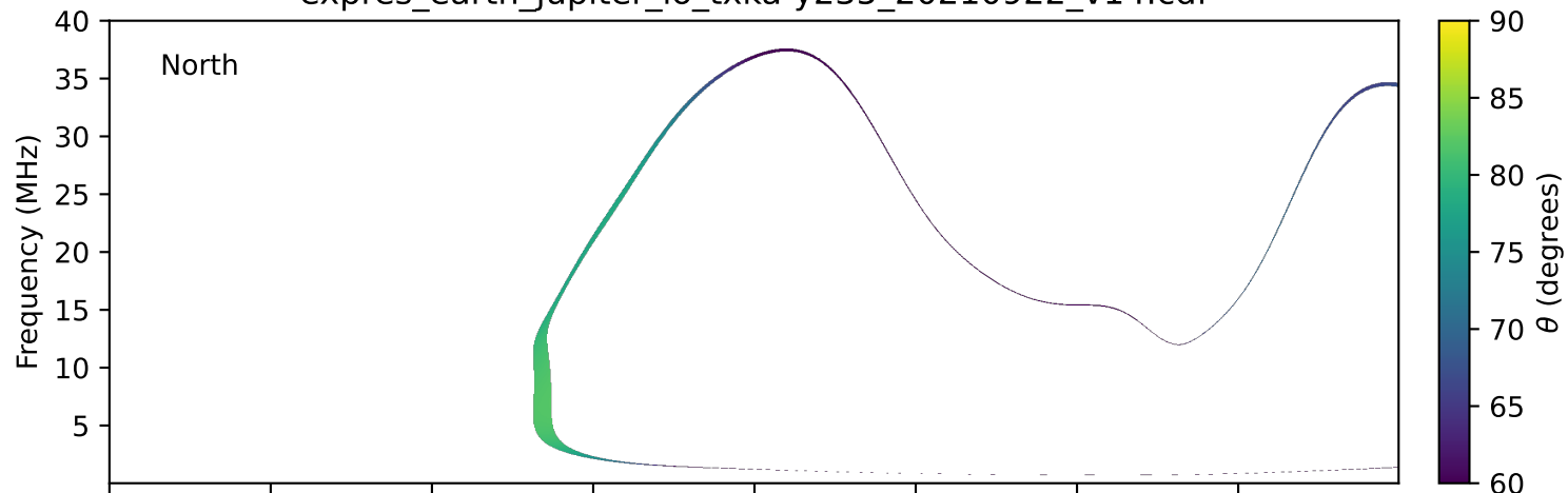
expres_earth_jupiter_io_txka-y235_20210922_v14.cdf
