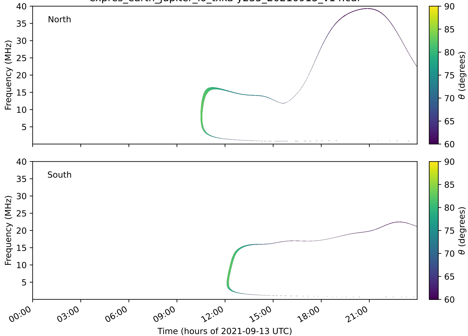
expres_earth_jupiter_io_txka-y235_20210913_v14.cdf
