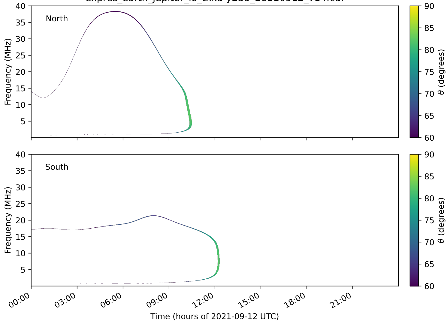
expres_earth_jupiter_io_txka-y235_20210912_v14.cdf
