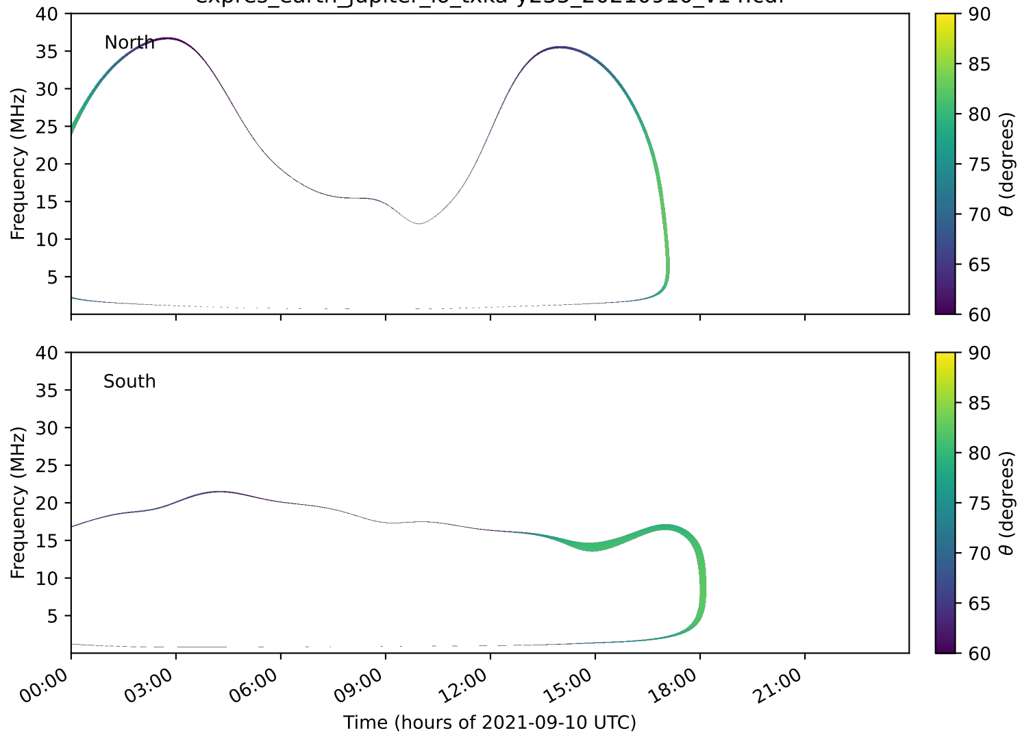
expres_earth_jupiter_io_txka-y235_20210910_v14.cdf
