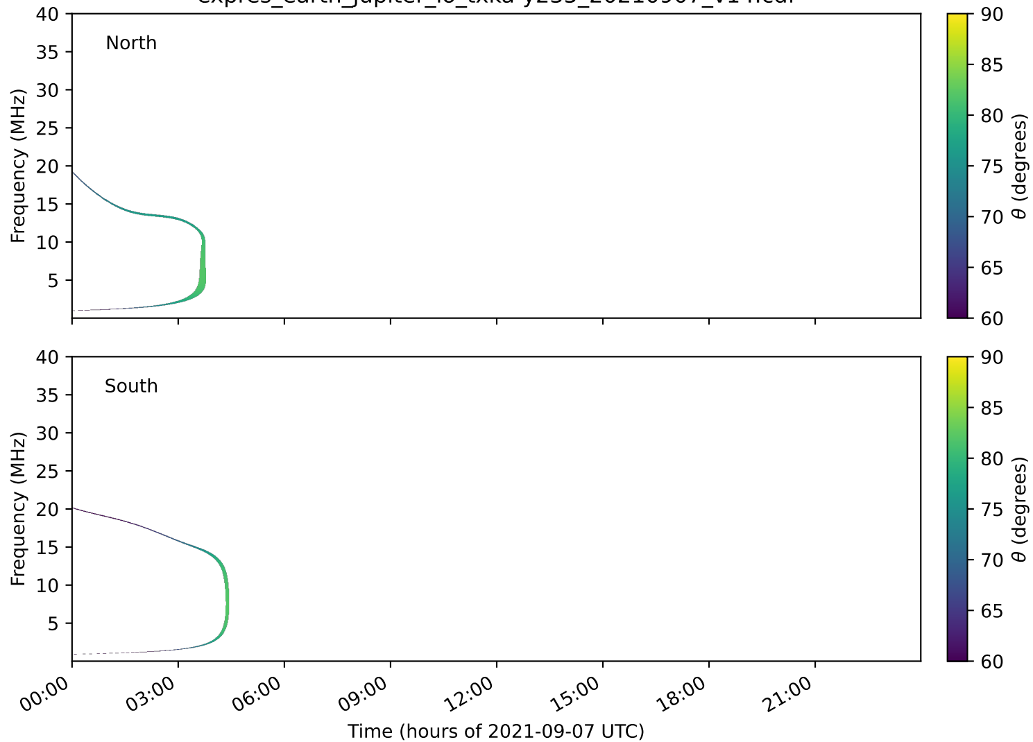
expres_earth_jupiter_io_txka-y235_20210907_v14.cdf
