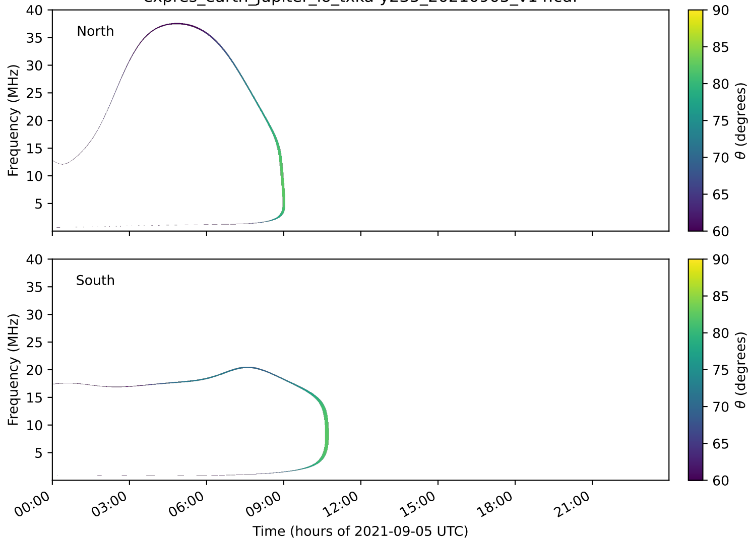
expres_earth_jupiter_io_txka-y235_20210905_v14.cdf
