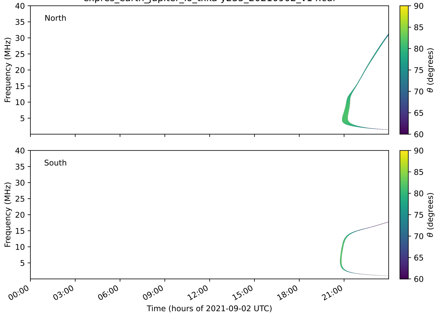
expres_earth_jupiter_io_txka-y235_20210902_v14.cdf
