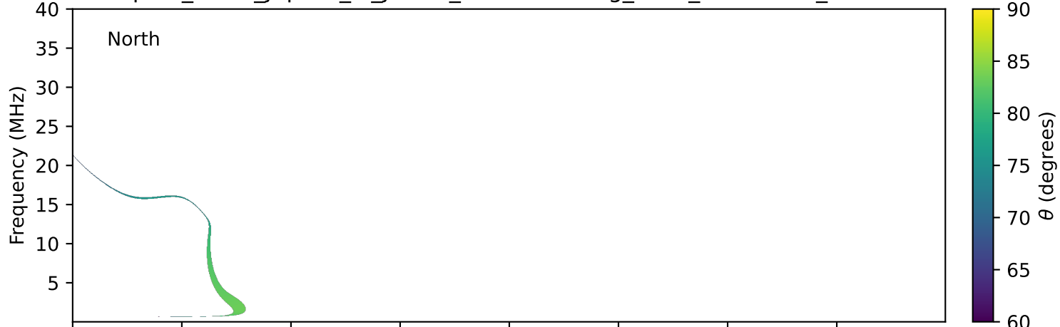
expres_earth_jupiter_io_jrm33_lossc-wid1deg_3kev_20210907_v11.cdf
