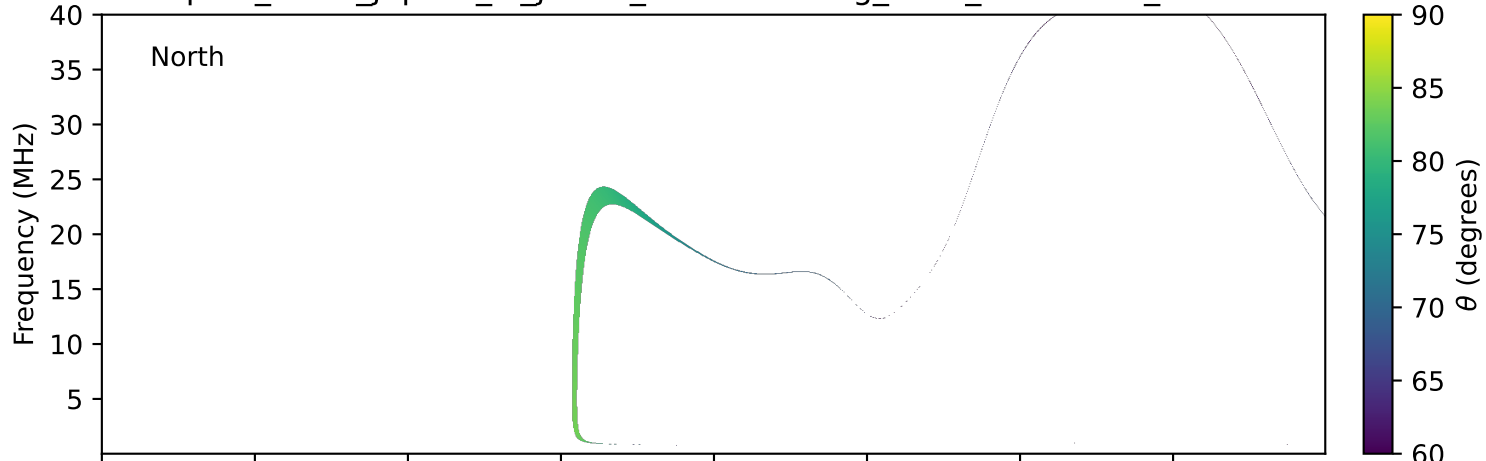
expres_earth_jupiter_io_jrm33_lossc-wid1deg_3kev_20210906_v11.cdf
