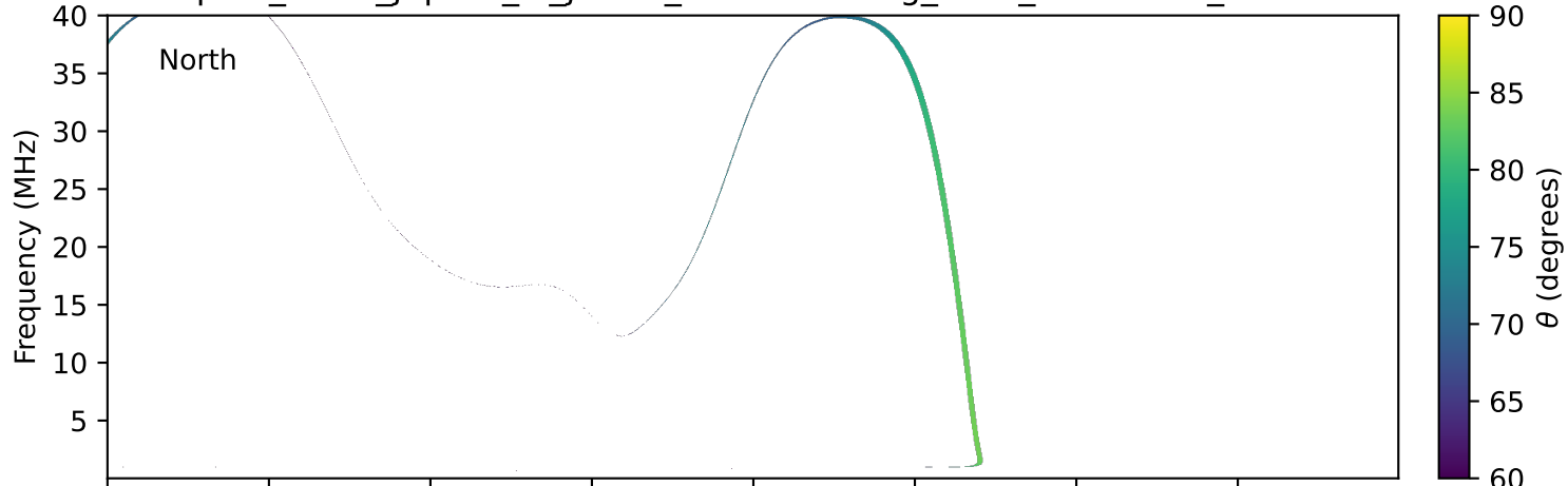
expres_earth_jupiter_io_jrm33_lossc-wid1deg_3kev_20210903_v11.cdf
