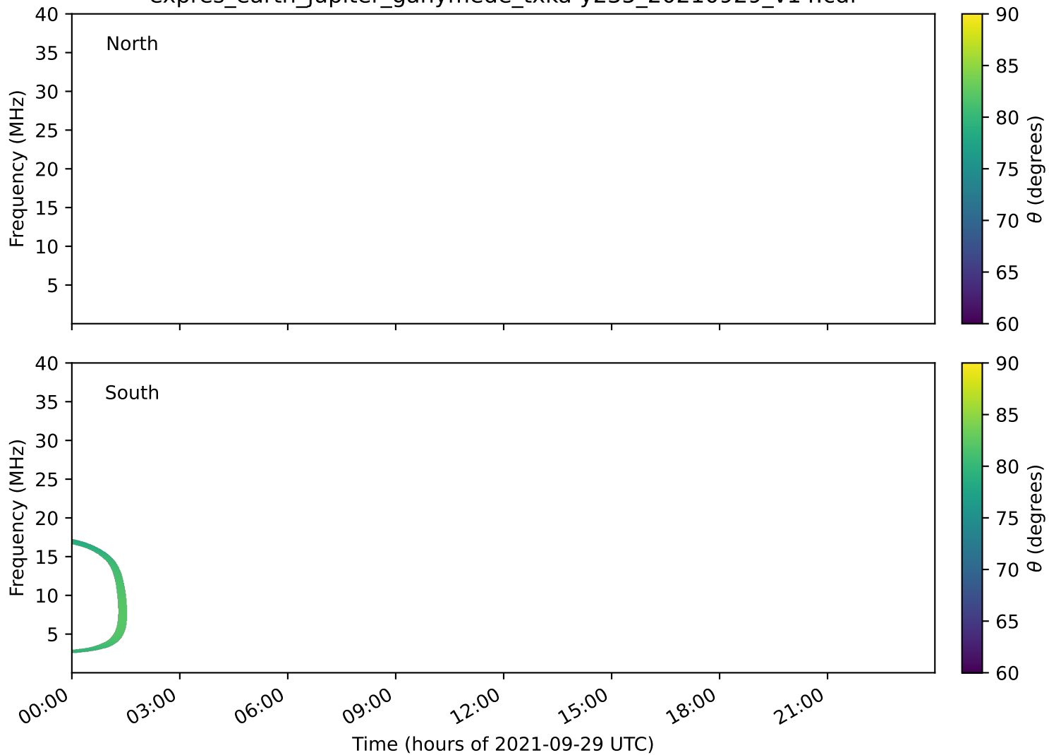
expres_earth_jupiter_ganymede_txka-y235_20210929_v14.cdf
