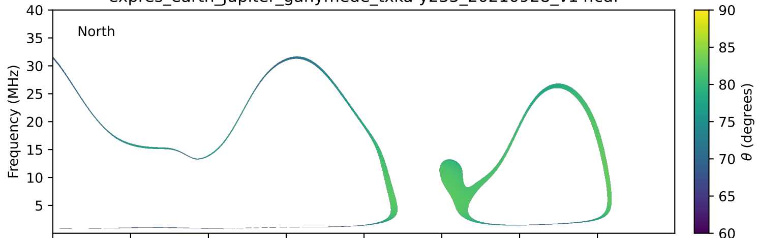
expres_earth_jupiter_ganymede_txka-y235_20210928_v14.cdf
