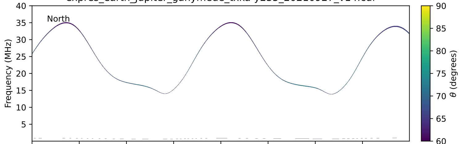
expres_earth_jupiter_ganymede_txka-y235_20210927_v14.cdf
