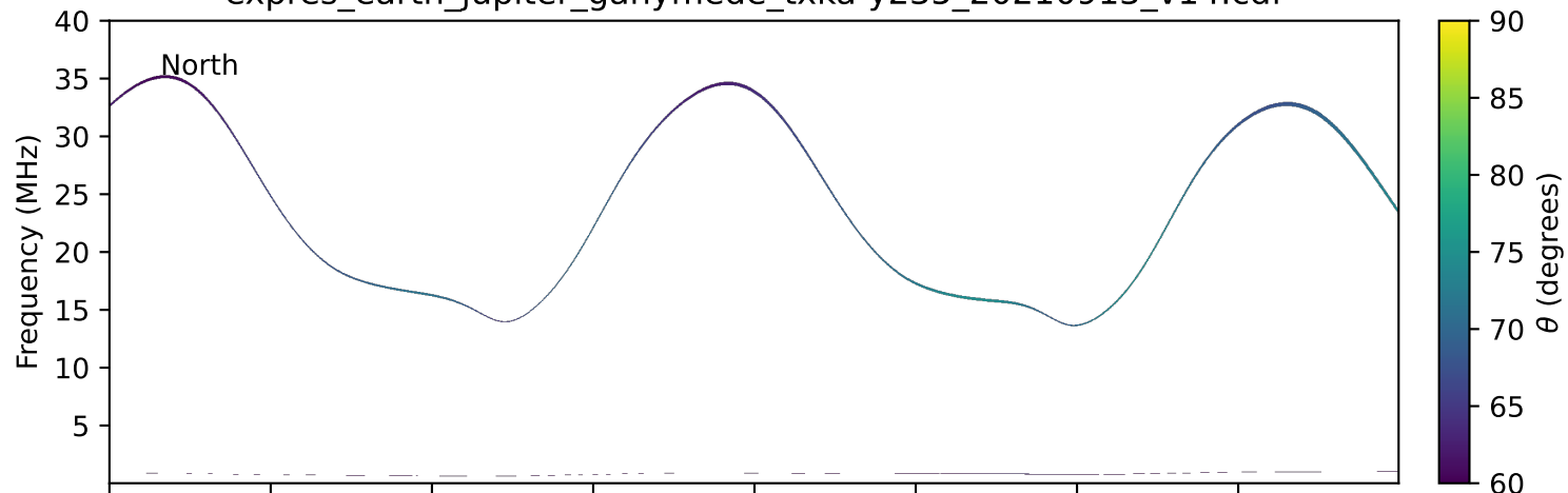
expres_earth_jupiter_ganymede_txka-y235_20210913_v14.cdf
