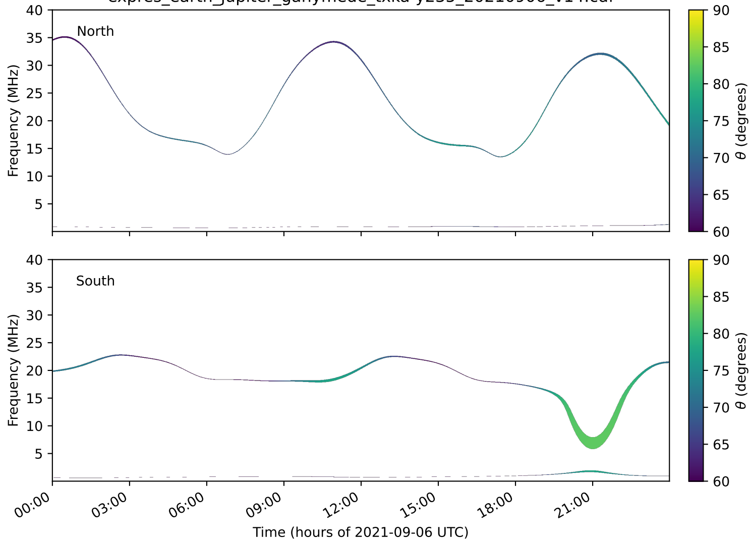
expres_earth_jupiter_ganymede_txka-y235_20210906_v14.cdf
