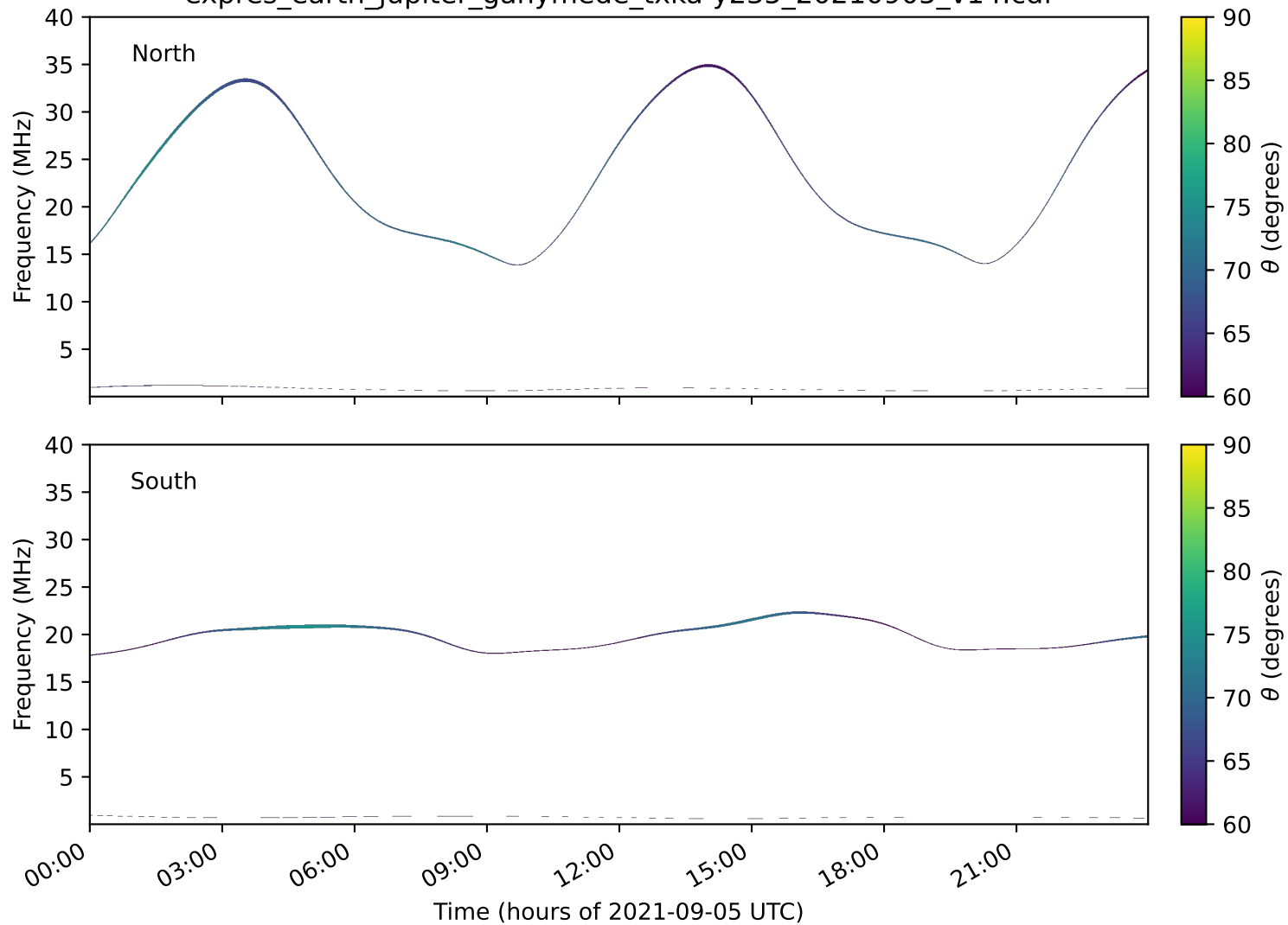
expres_earth_jupiter_ganymede_txka-y235_20210905_v14.cdf
