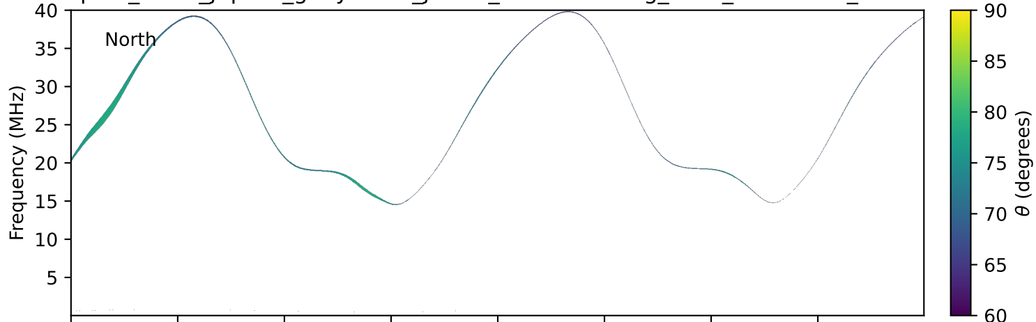
expres_earth_jupiter_ganymede_jrm33_lossc-wid1deg_3kev_20210905_v11.cdf
