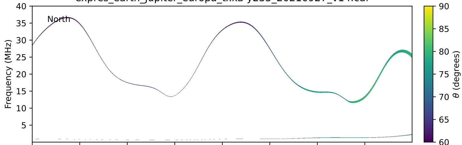
expres_earth_jupiter_europa_txka-y235_20210927_v14.cdf
