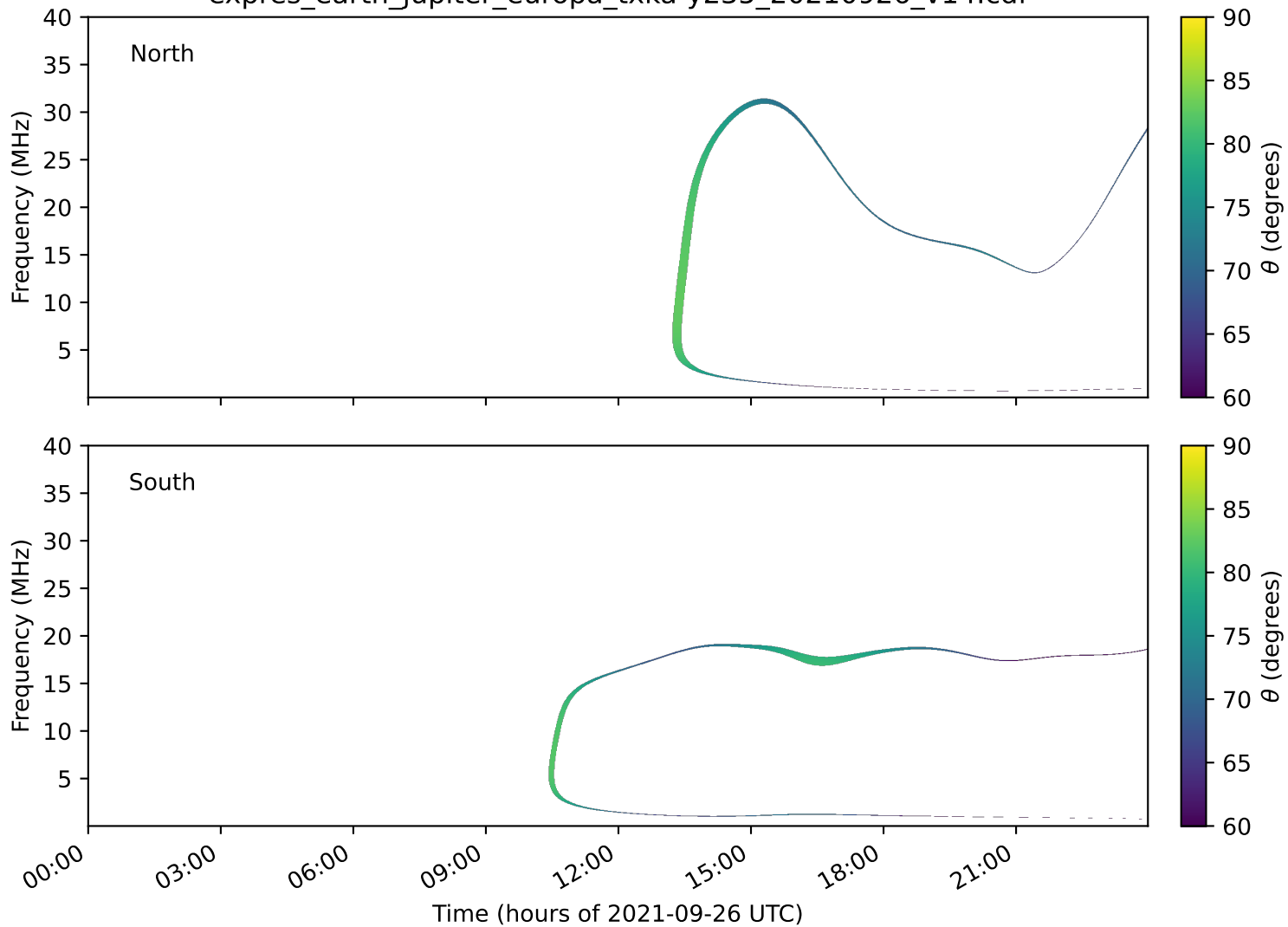
expres_earth_jupiter_europa_txka-y235_20210926_v14.cdf
