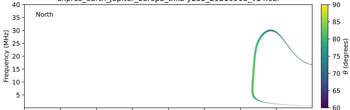
expres_earth_jupiter_europa_txka-y235_20210908_v14.cdf
