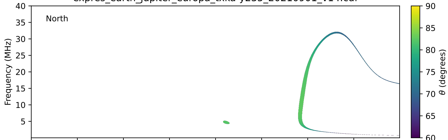
expres_earth_jupiter_europa_txka-y235_20210901_v14.cdf
