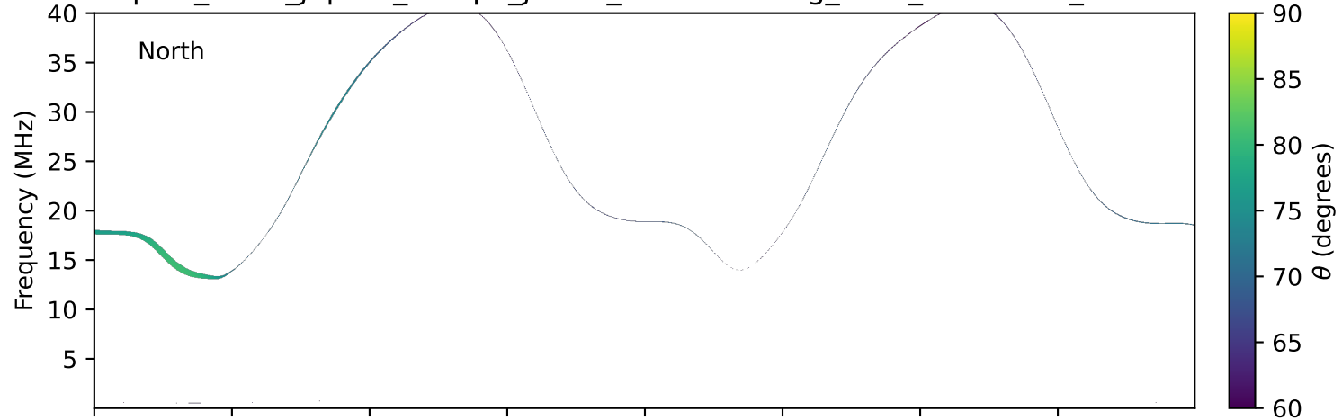
expres_earth_jupiter_europa_jrm33_lossc-wid1deg_3kev_20210916_v11.cdf
