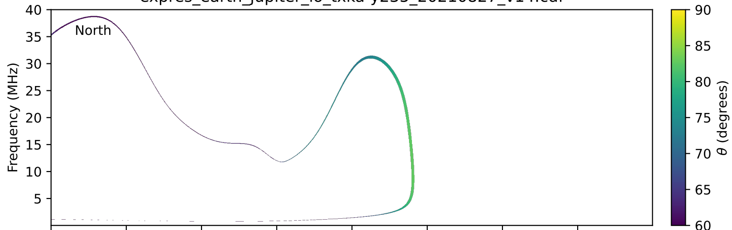
expres_earth_jupiter_io_txka-y235_20210827_v14.cdf
